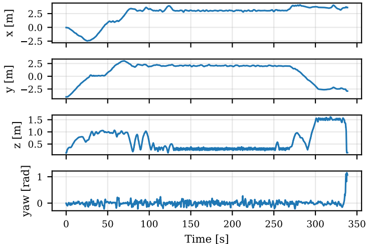
exp 5 - UAV 1 - Position
